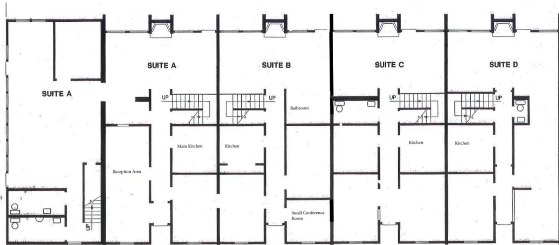
GROUND LEVEL FLOOR PLAN
